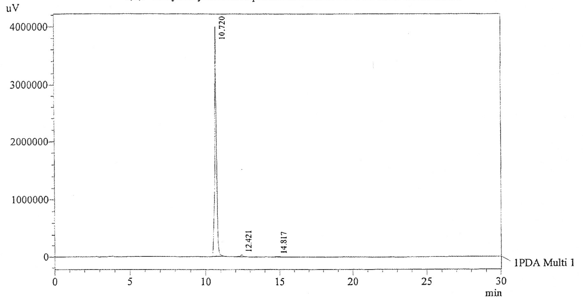
Chromatogram 6,7,3'-Trihydroxyflavone D:\promonence\Data\2013\FEB-2013\020213H.lcd
